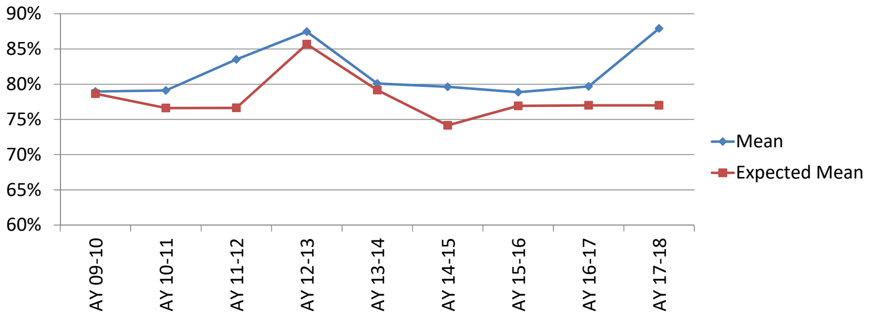
Mean vs. Expected Mean
