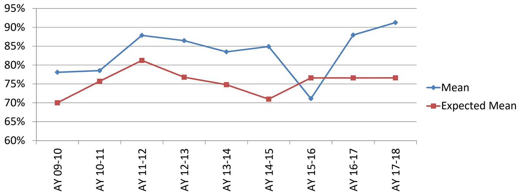
Mean vs. Expected Mean
